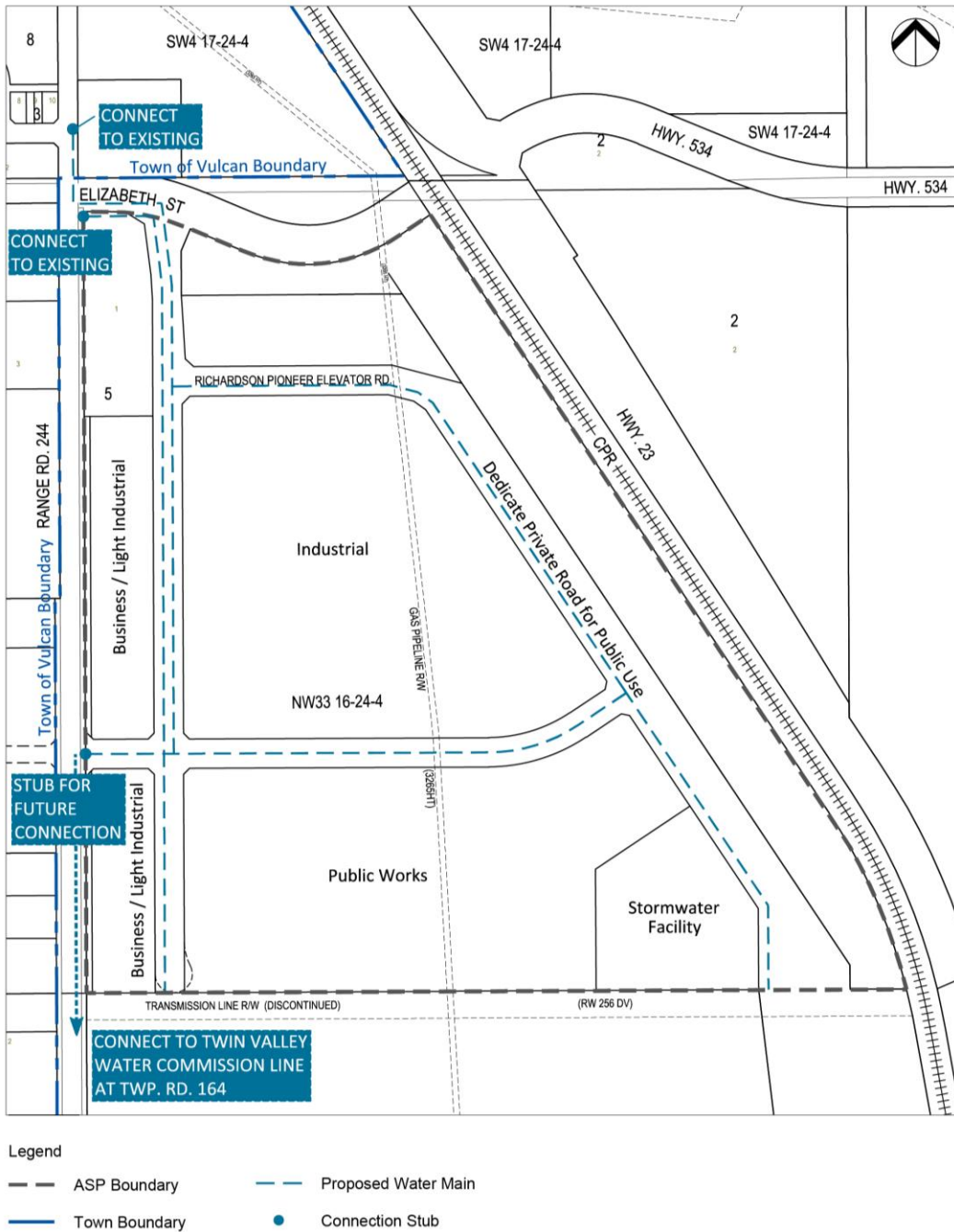
Figure 7 - Water Servicing Plan
